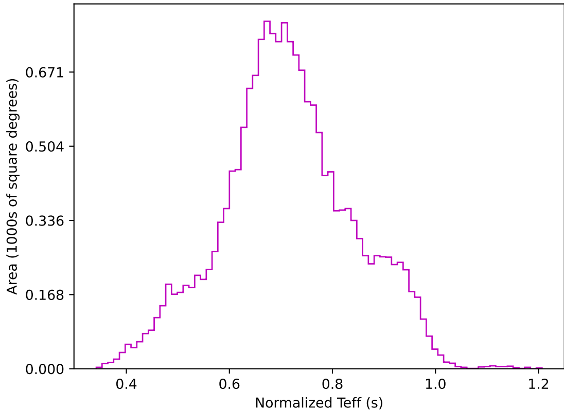
ddf_acor_sf25_lsf40_lsr10_v3.4_10yrs WFD z band: Normalized Teff
