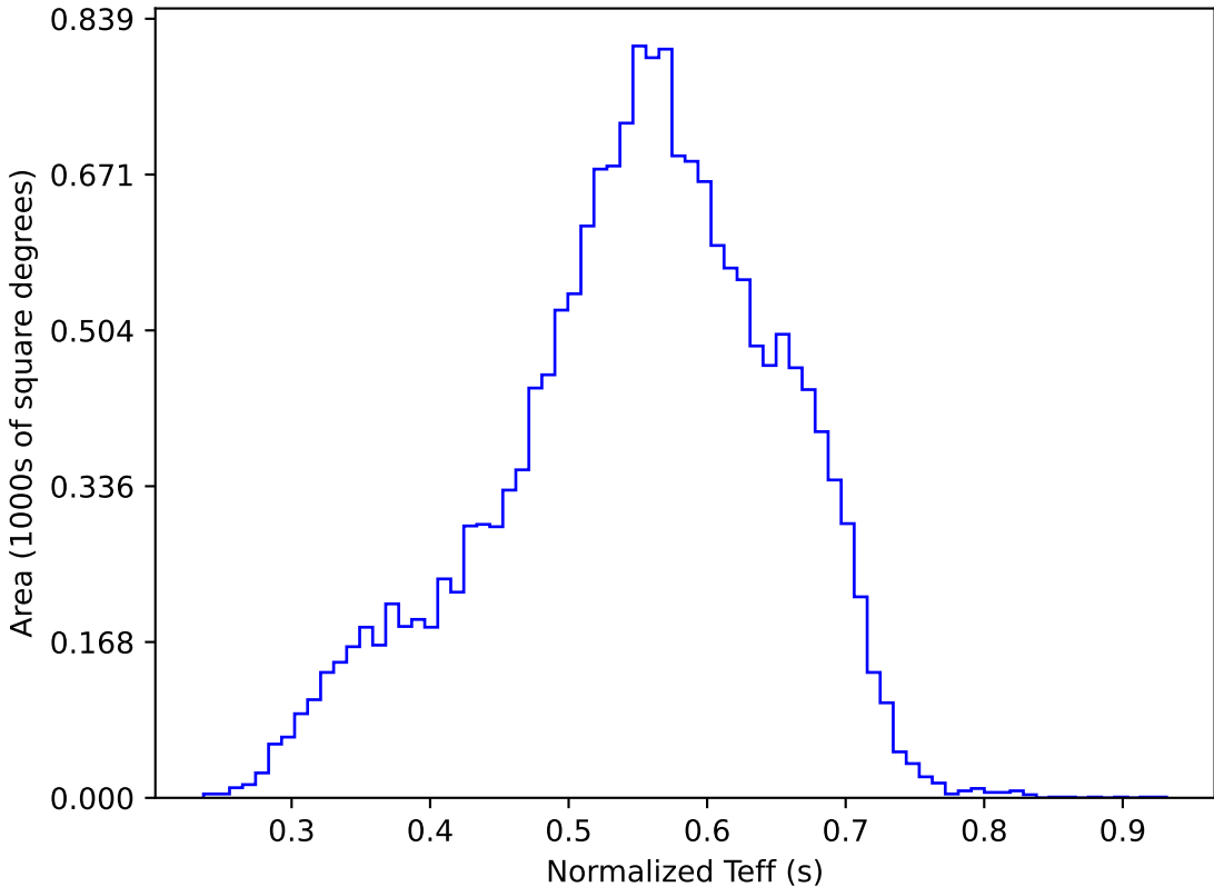
ddf_acor_sf25_lsf40_lsr10_v3.4_10yrs WFD y band: Normalized Teff
