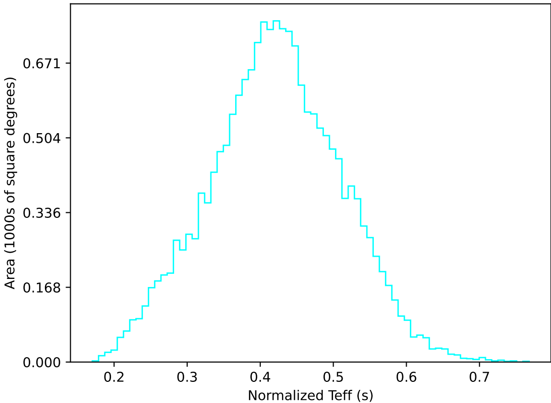
ddf_acor_sf25_lsf40_lsr10_v3.4_10yrs WFD u band: Normalized Teff
