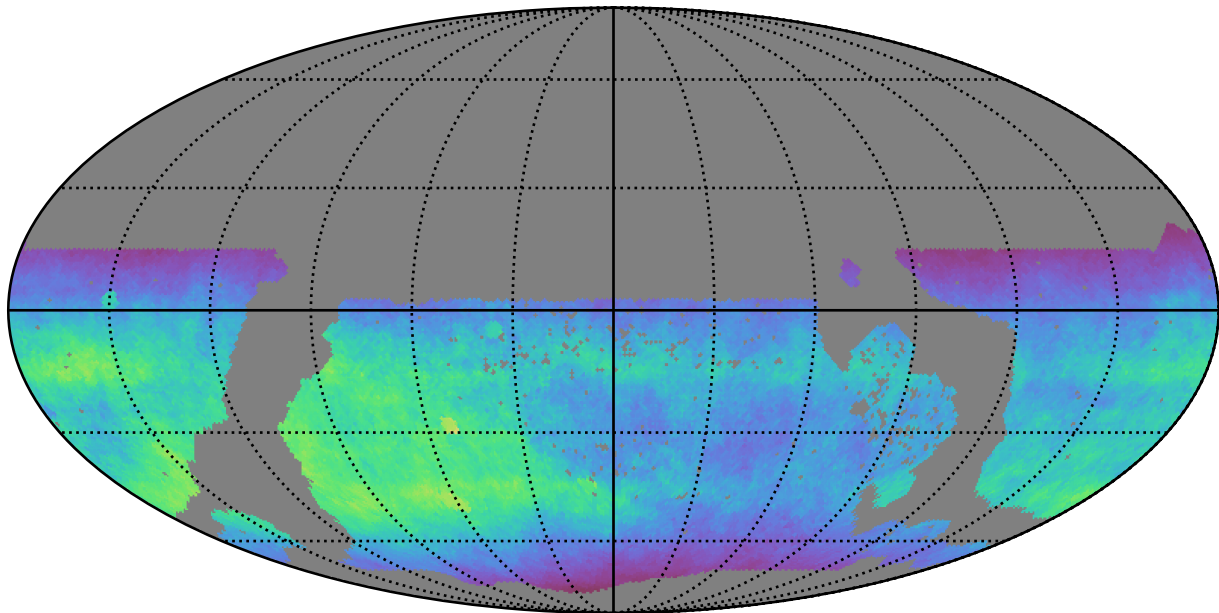
ddf_acor_sf25_lsf40_lsr10_v3.4_10yrs WFD i band: Normalized Teff
