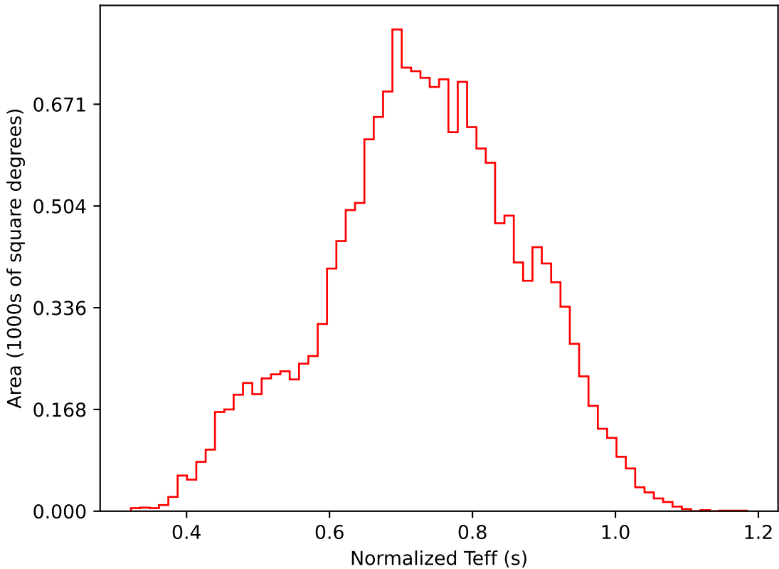
ddf_acor_sf25_lsf40_lsr10_v3.4_10yrs WFD i band: Normalized Teff
