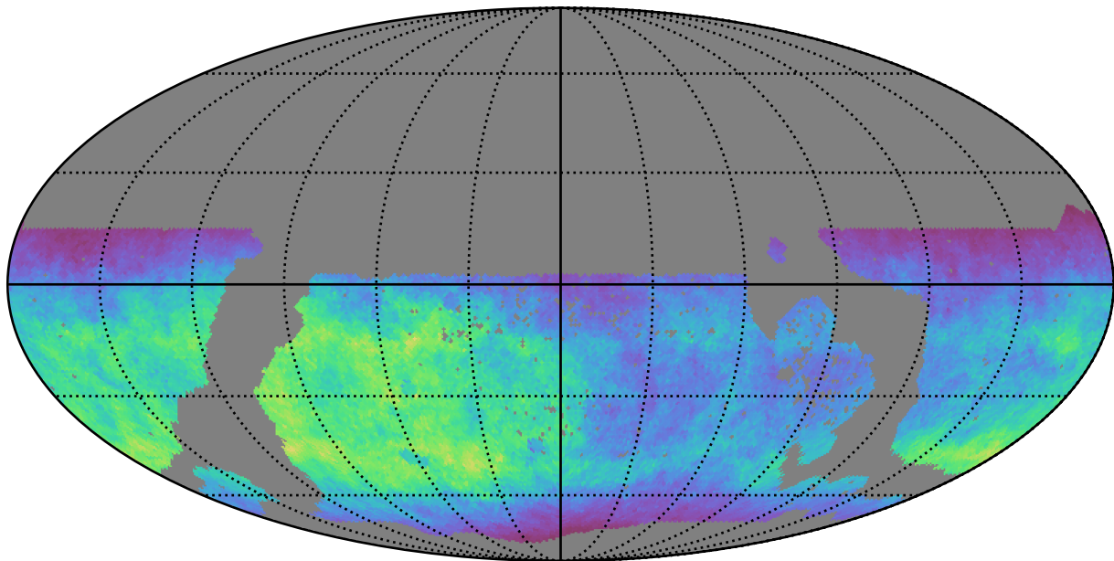
ddf_acor_sf25_lsf40_lsr10_v3.4_10yrs WFD g band: Normalized Teff
