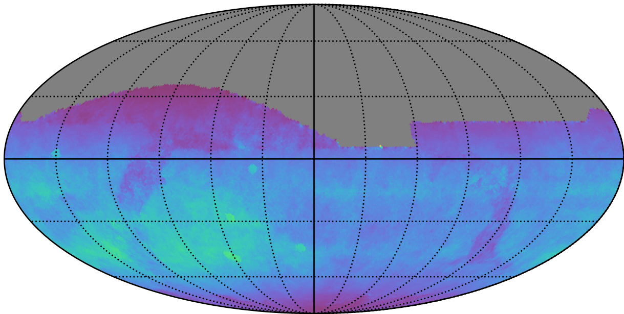
ddf_acor_sf25_lsf40_lsr10_v3.4_10yrs All sky z band: Normalized Teff
