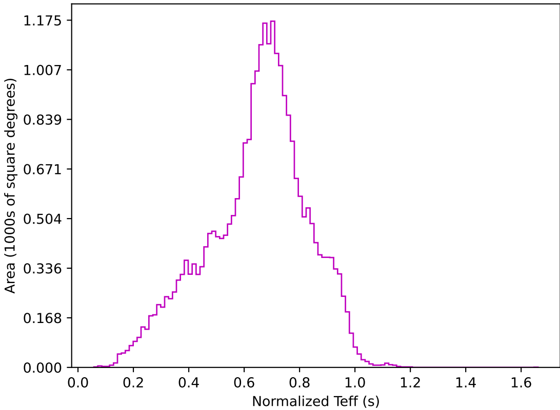
ddf_acor_sf25_lsf40_lsr10_v3.4_10yrs All sky z band: Normalized Teff
