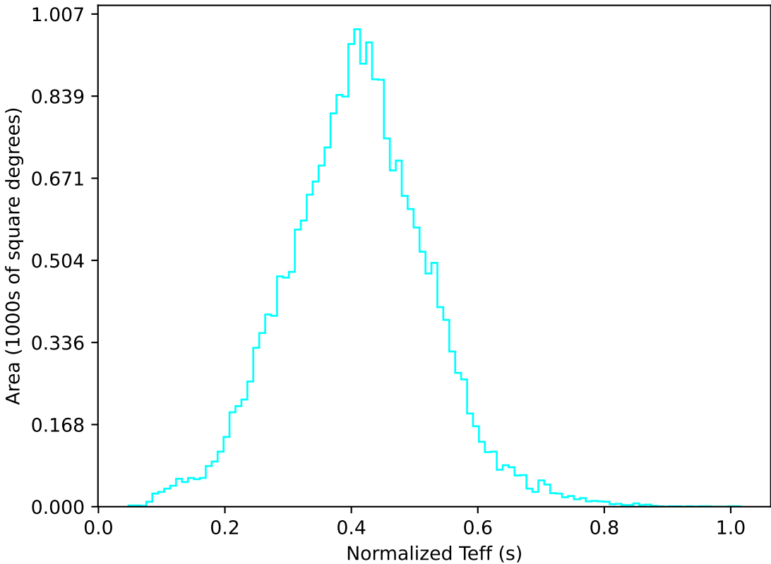
ddf_acor_sf25_lsf40_lsr10_v3.4_10yrs All sky u band: Normalized Teff
