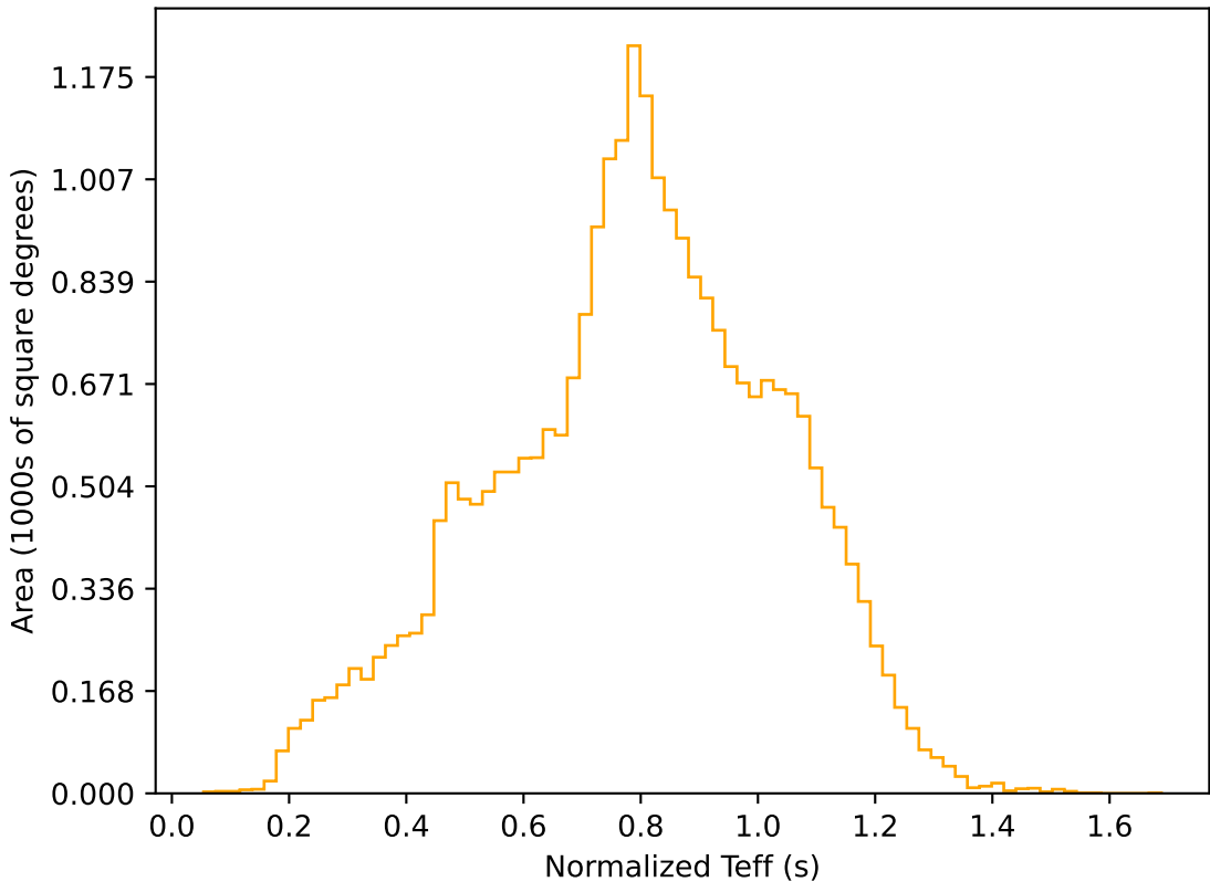
ddf_acor_sf25_lsf40_lsr10_v3.4_10yrs All sky r band: Normalized Teff
