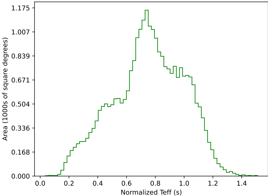
ddf_acor_sf25_lsf40_lsr10_v3.4_10yrs All sky g band: Normalized Teff
