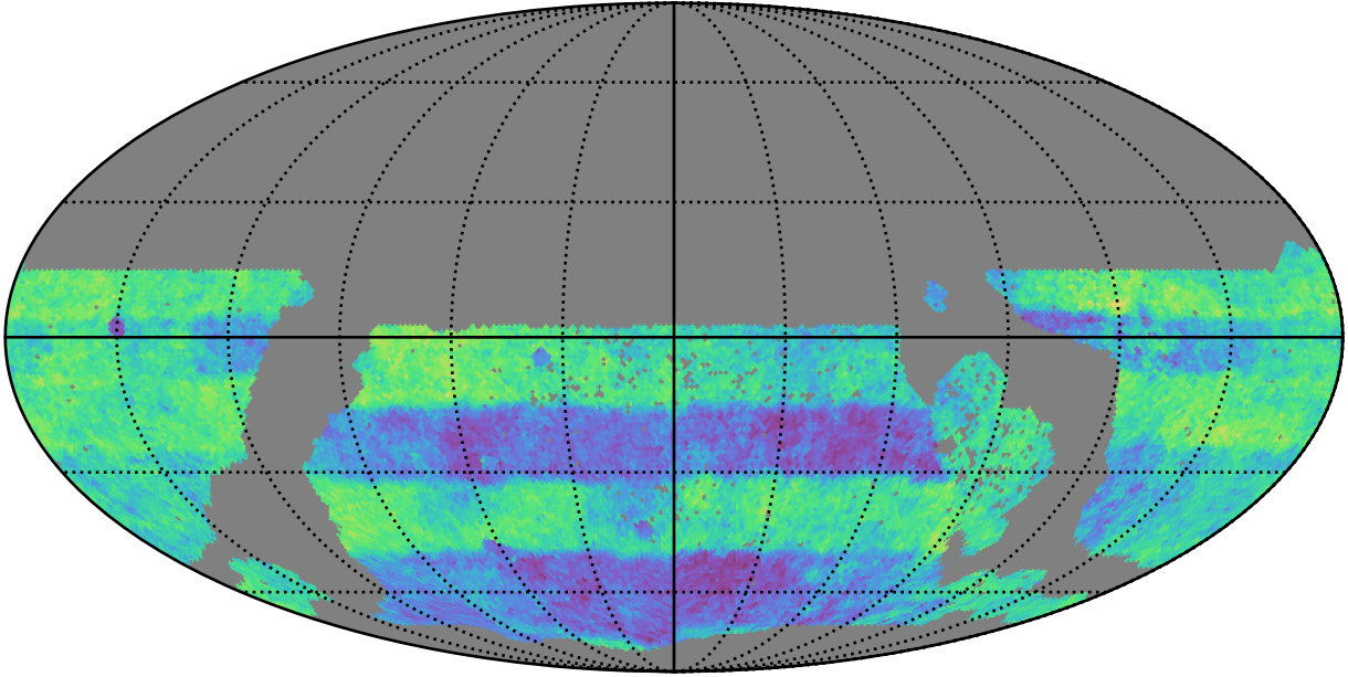
ddf_acor_sf25_lsf40_lsr10_v3.4_10yrs WFD: Normalized Proper Motion Uncert @ 24.0
