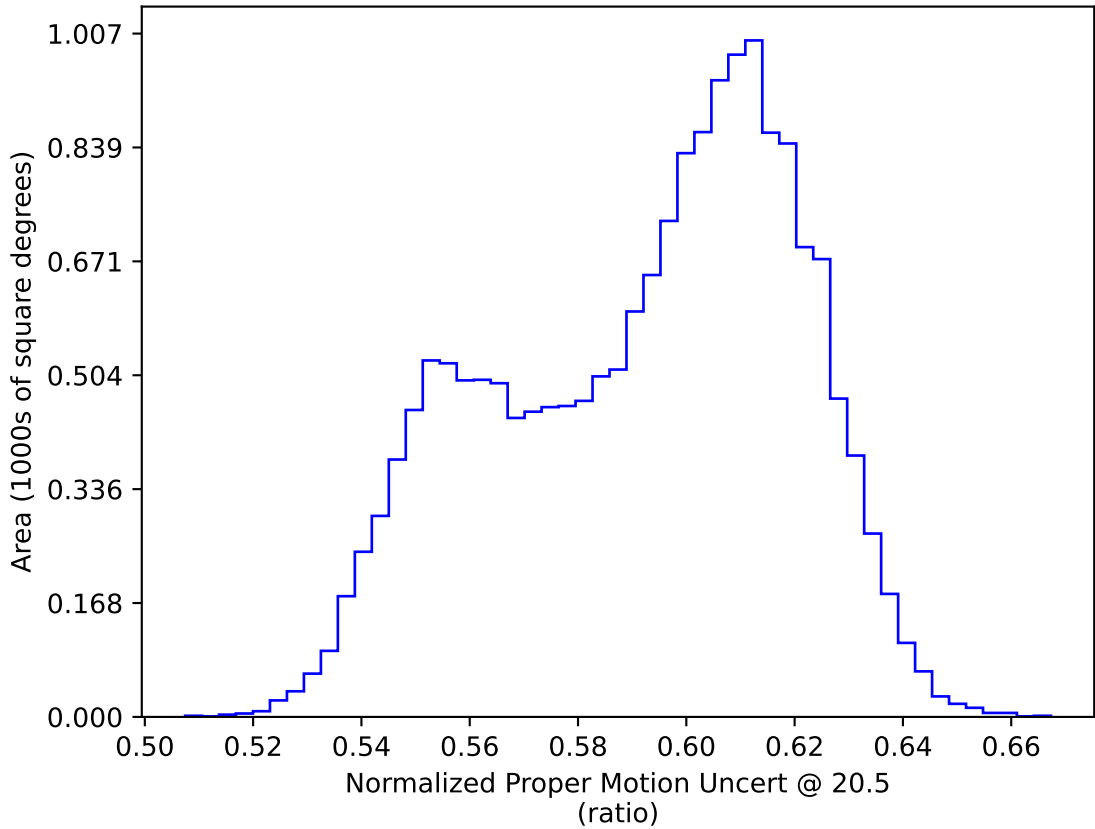
ddf_acor_sf25_lsf40_lsr10_v3.4_10yrs WFD: Normalized Proper Motion Uncert @ 20.5
