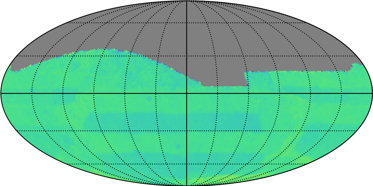
ddf_acor_sf25_lsf40_lsr10_v3.4_10yrs All sky: Normalized Proper Motion Uncert @ 20.5
