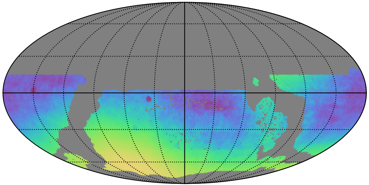
ddf_acor_sf25_lsf40_lsr10_v3.4_10yrs WFD: Normalized Parallax Uncert @ 24.0
