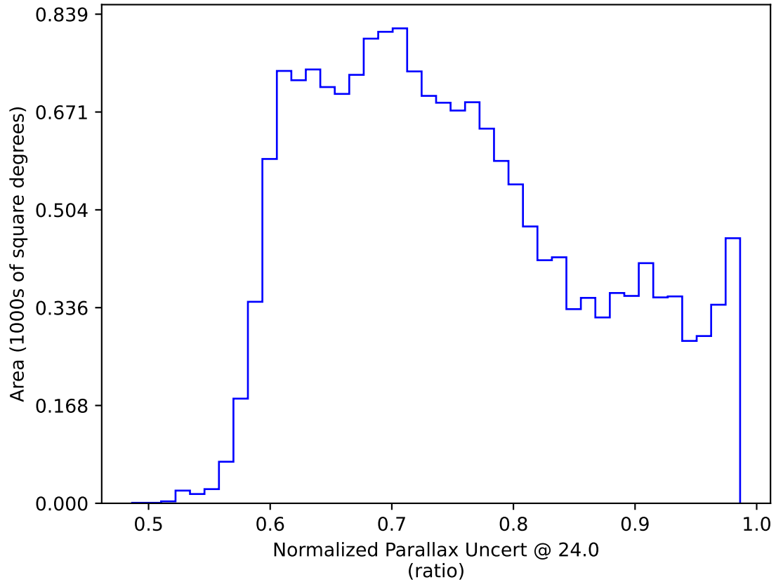
ddf_acor_sf25_lsf40_lsr10_v3.4_10yrs WFD: Normalized Parallax Uncert @ 24.0
