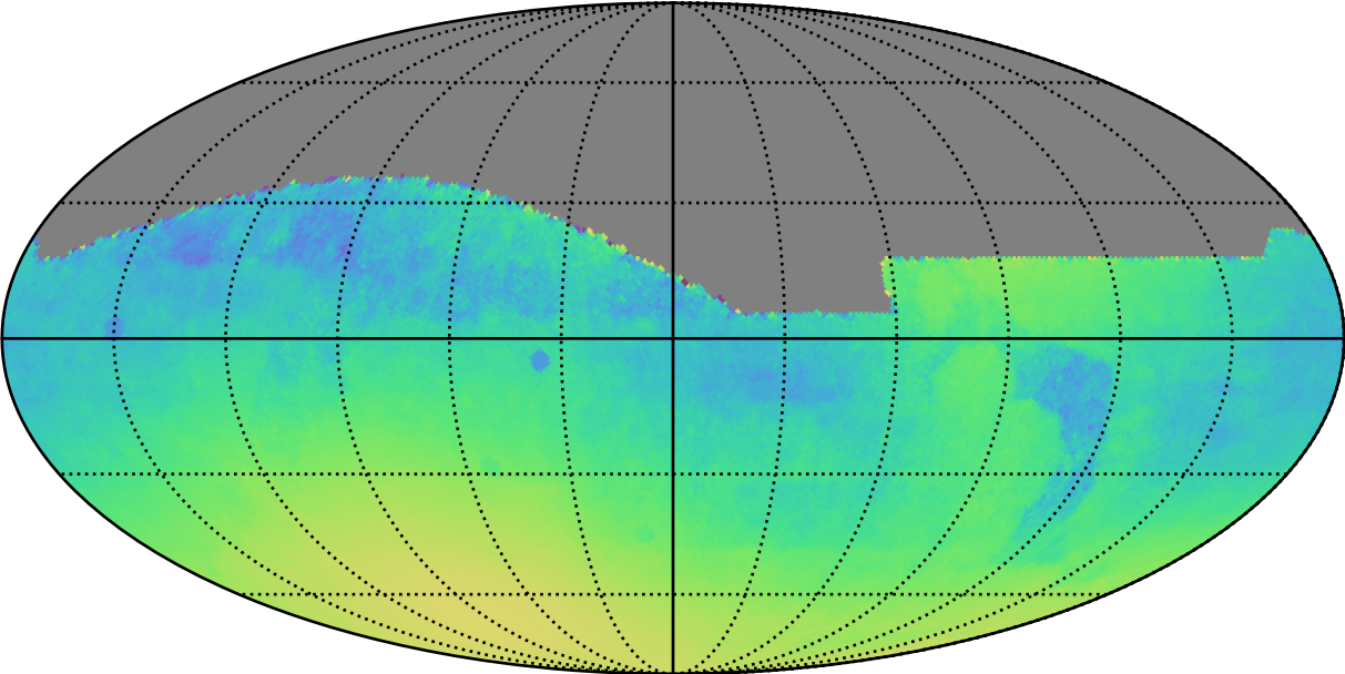
ddf_acor_sf25_lsf40_lsr10_v3.4_10yrs All sky: Normalized Parallax Uncert @ 24.0
