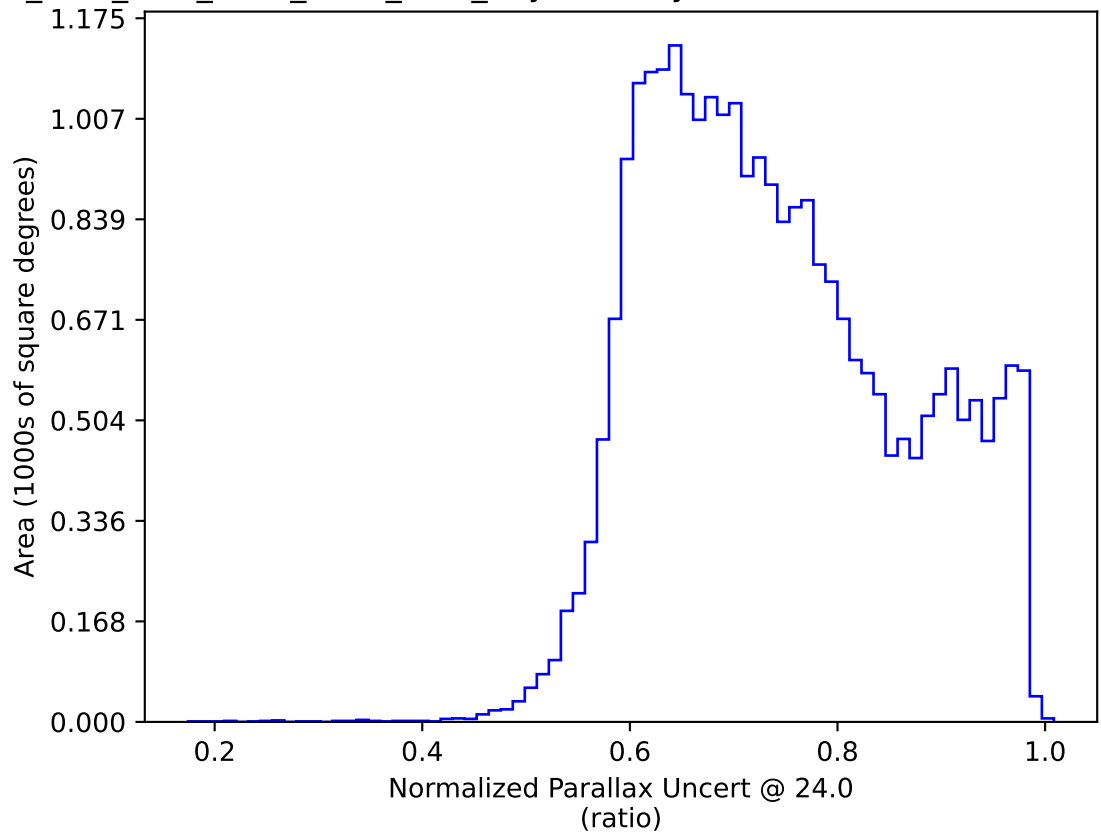
ddf_acor_sf25_lsf40_lsr10_v3.4_10yrs All sky: Normalized Parallax Uncert @ 24.0
