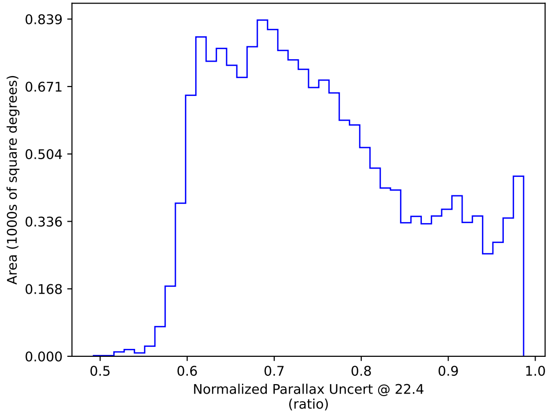
ddf_acor_sf25_lsf40_lsr10_v3.4_10yrs WFD: Normalized Parallax Uncert @ 22.4
