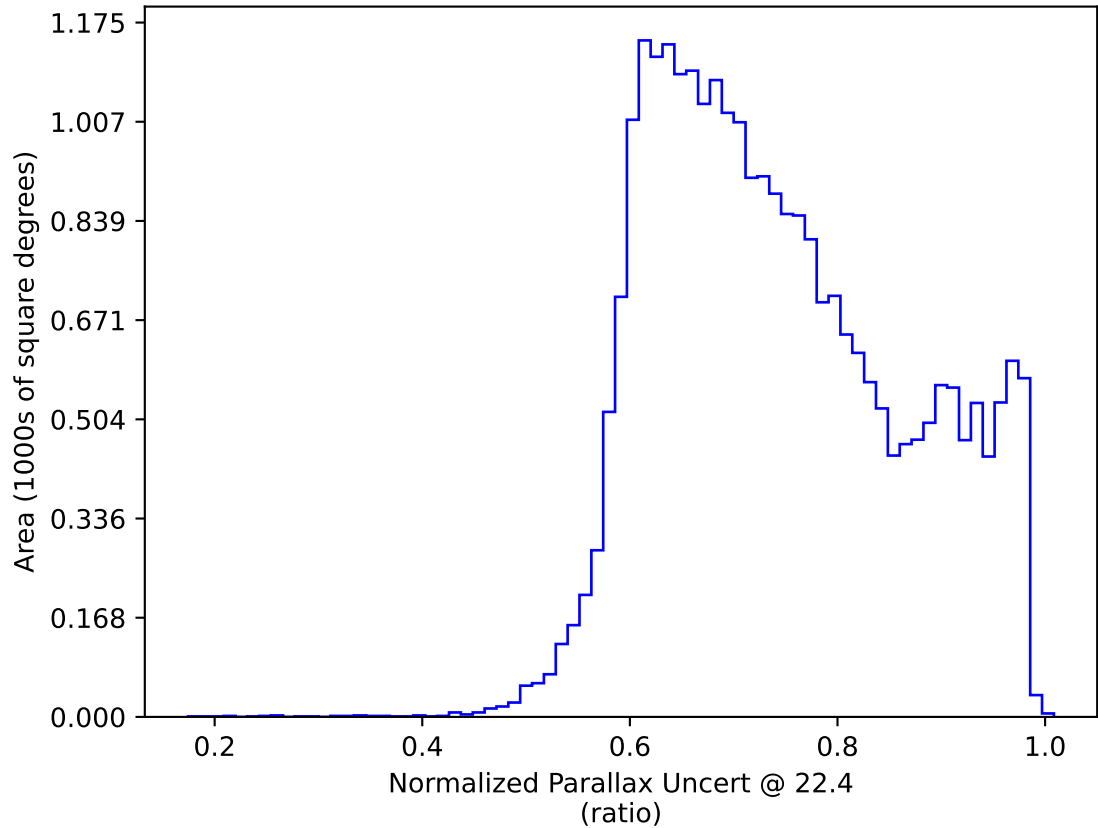
ddf_acor_sf25_lsf40_lsr10_v3.4_10yrs All sky: Normalized Parallax Uncert @ 22.4
