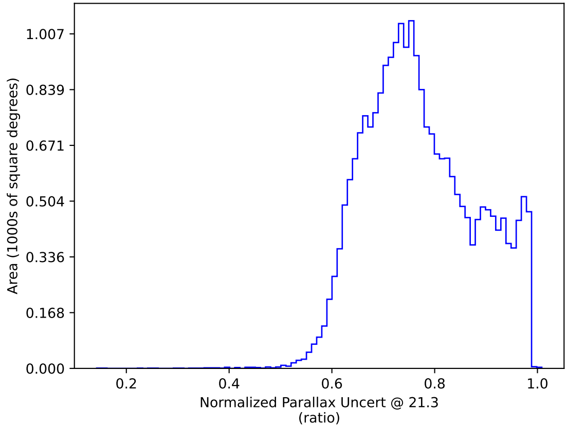
ddf_acor_sf25_lsf40_lsr10_v3.4_10yrs All sky y band only: Normalized Parallax Uncert @ 21.3
