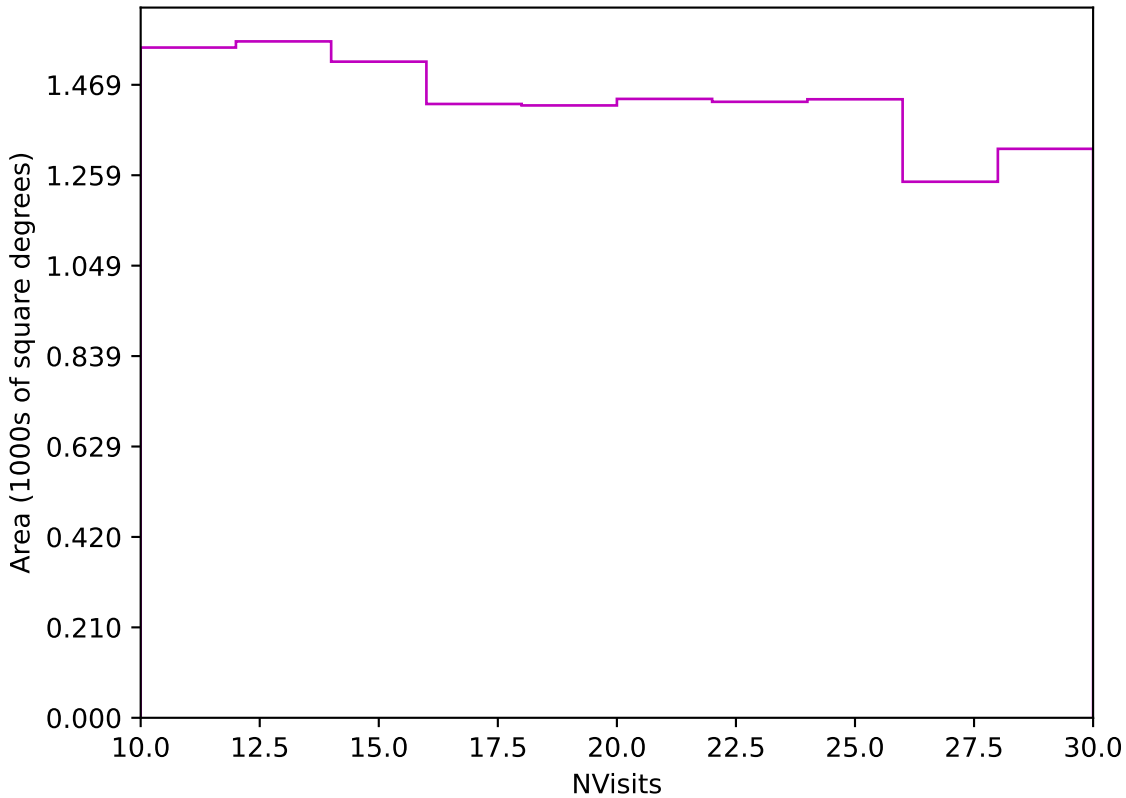
ddf_acor_sf25_lsf40_lsr10_v3.4_10yrs Yr 3-4 z band: NVisits
