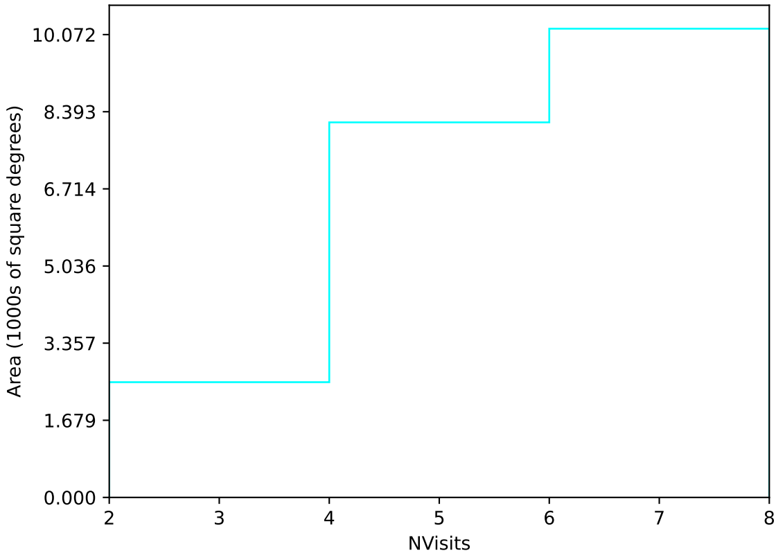
ddf_acor_sf25_lsf40_lsr10_v3.4_10yrs Yr 1 u band: NVisits
