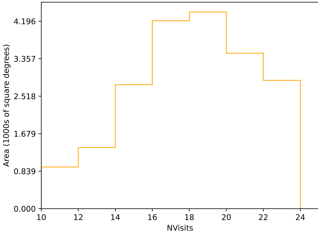
ddf_acor_sf25_lsf40_lsr10_v3.4_10yrs Yr 1 r band: NVisits
