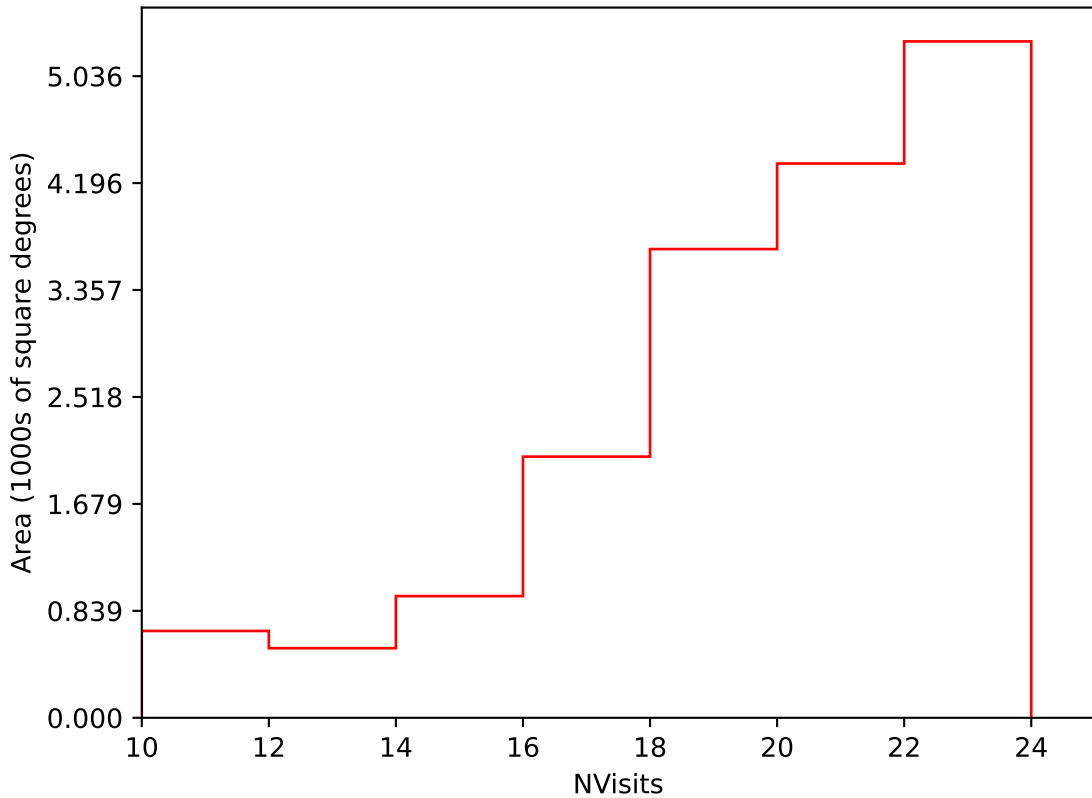
ddf_acor_sf25_lsf40_lsr10_v3.4_10yrs Yr 1 i band: NVisits
