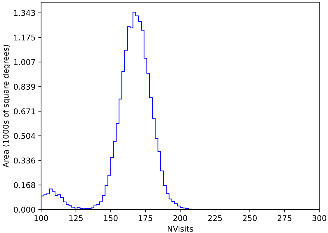
ddf_acor_sf25_lsf40_lsr10_v3.4_10yrs WFD y band: NVisits
