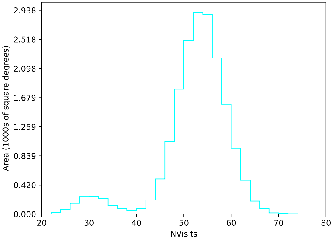
ddf_acor_sf25_lsf40_lsr10_v3.4_10yrs WFD u band: NVisits
