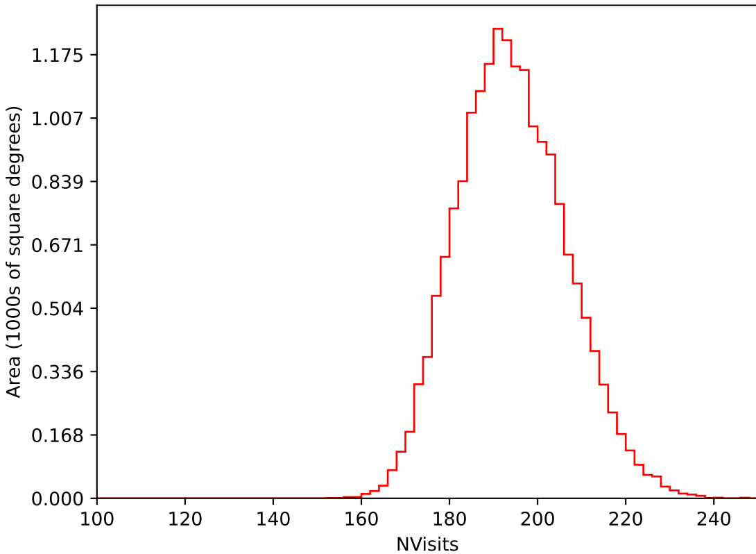
ddf_acor_sf25_lsf40_lsr10_v3.4_10yrs WFD i band: NVisits
