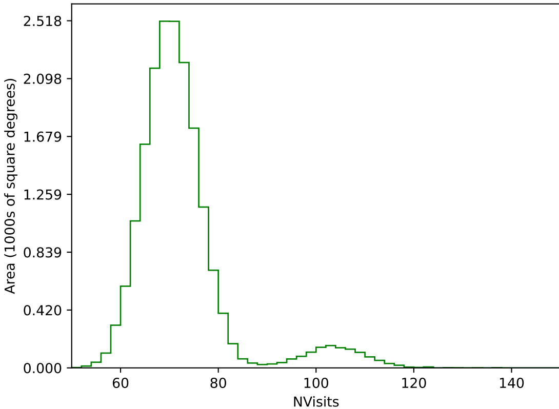
ddf_acor_sf25_lsf40_lsr10_v3.4_10yrs WFD g band: NVisits
