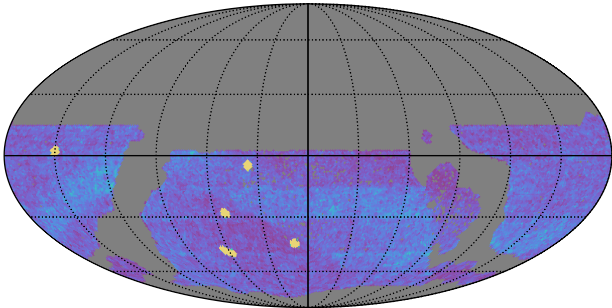
ddf_acor_sf25_lsf40_lsr10_v3.4_10yrs WFD all bands: NVisits
