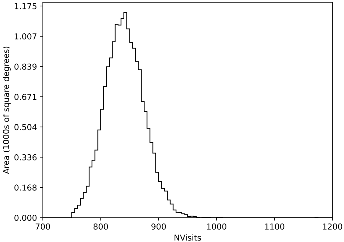
ddf_acor_sf25_lsf40_lsr10_v3.4_10yrs WFD all bands: NVisits
