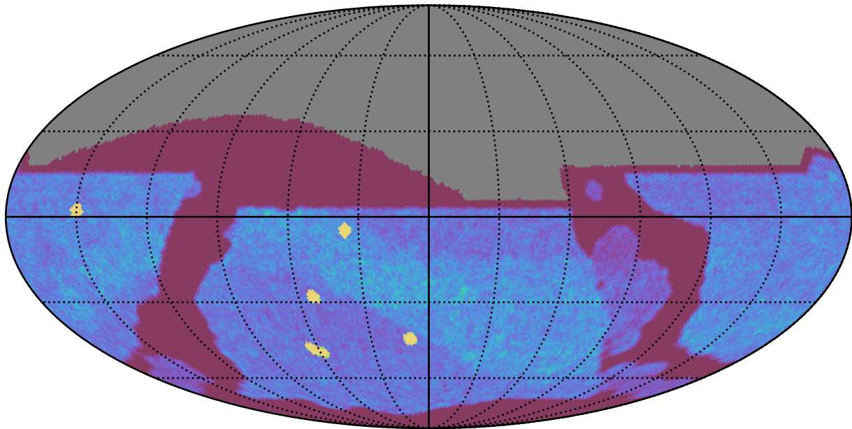
ddf_acor_sf25_lsf40_lsr10_v3.4_10yrs All sky z band: NVisits
