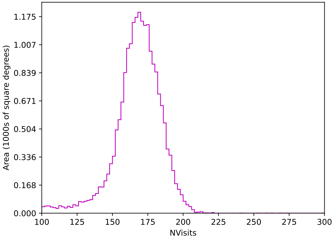
ddf_acor_sf25_lsf40_lsr10_v3.4_10yrs All sky z band: NVisits
