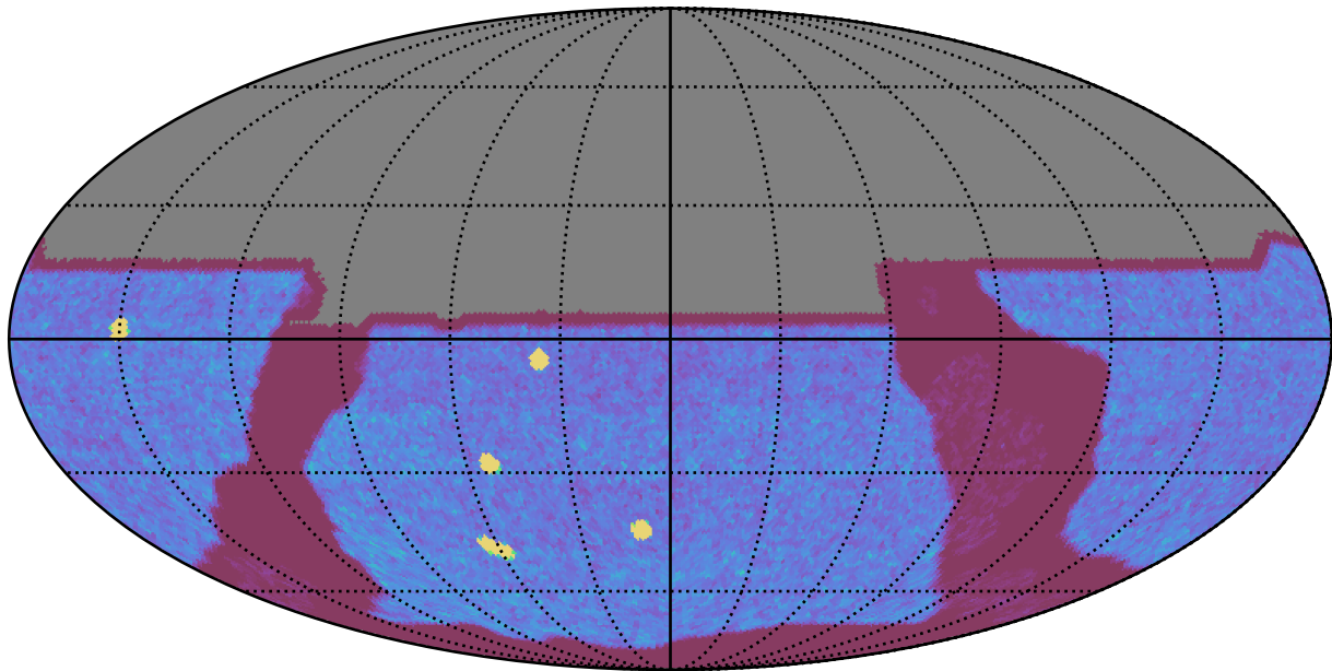
ddf_acor_sf25_lsf40_lsr10_v3.4_10yrs All sky y band: NVisits
