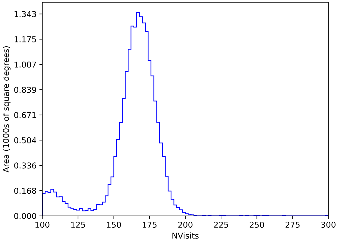
ddf_acor_sf25_lsf40_lsr10_v3.4_10yrs All sky y band: NVisits
