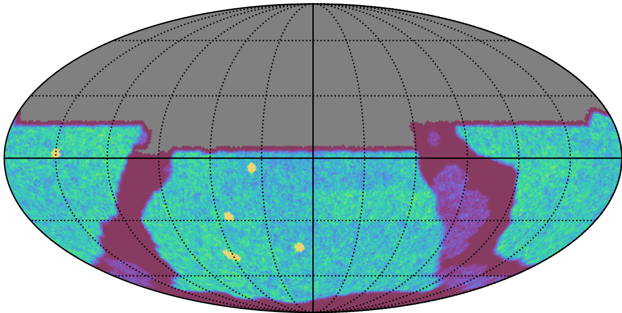
ddf_acor_sf25_lsf40_lsr10_v3.4_10yrs All sky u band: NVisits
