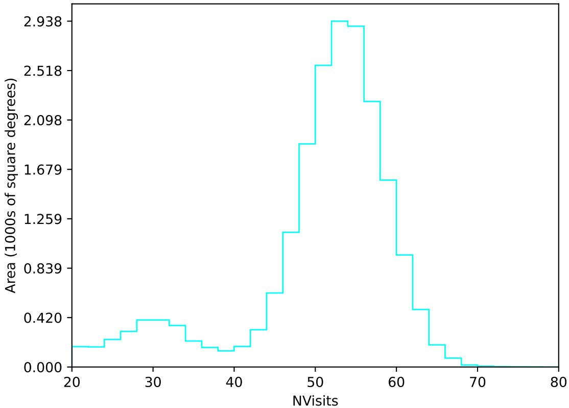
ddf_acor_sf25_lsf40_lsr10_v3.4_10yrs All sky u band: NVisits
