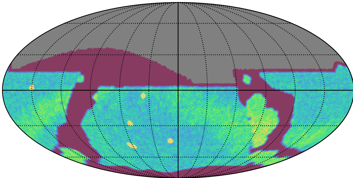
ddf_acor_sf25_lsf40_lsr10_v3.4_10yrs All sky r band: NVisits
