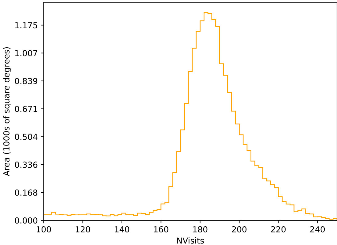
ddf_acor_sf25_lsf40_lsr10_v3.4_10yrs All sky r band: NVisits
