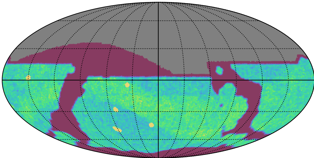
ddf_acor_sf25_lsf40_lsr10_v3.4_10yrs All sky i band: NVisits
