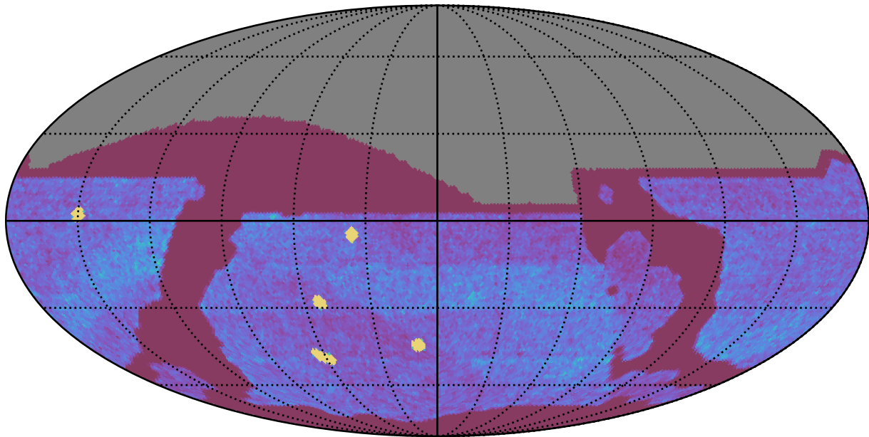
ddf_acor_sf25_lsf40_lsr10_v3.4_10yrs All sky all bands: NVisits
