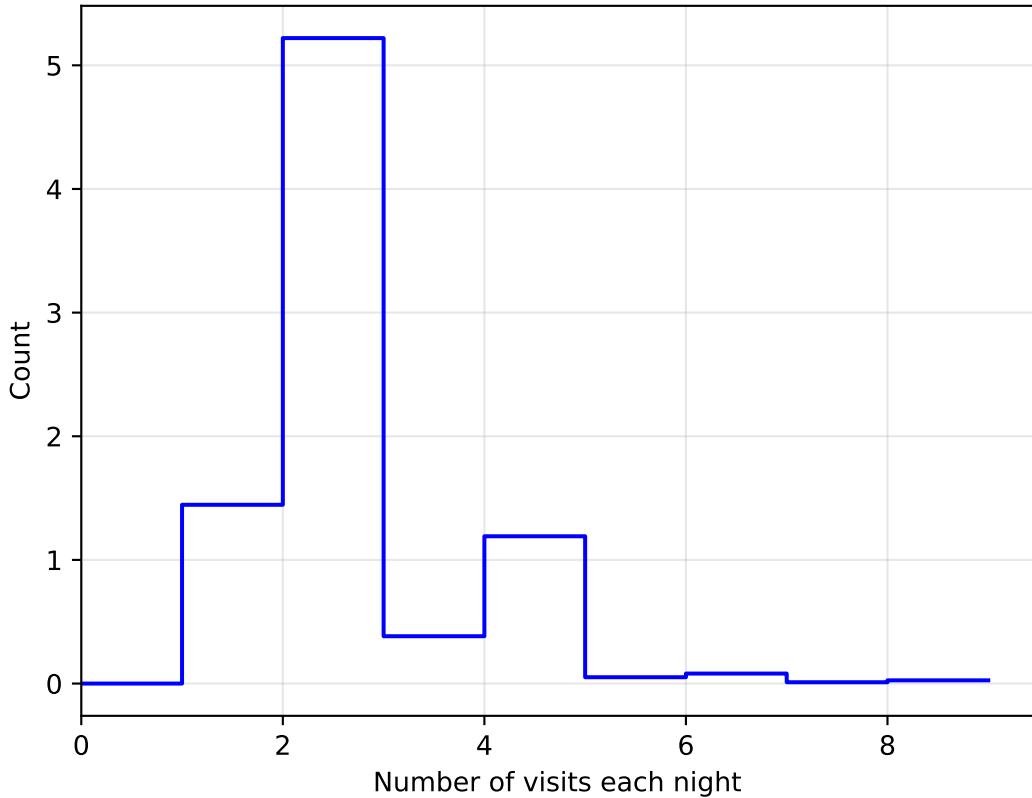
ddf_acor_sf25_lsf40_lsr10_v3.4_10yrs WFD: NVisitsPerNight 1e6
