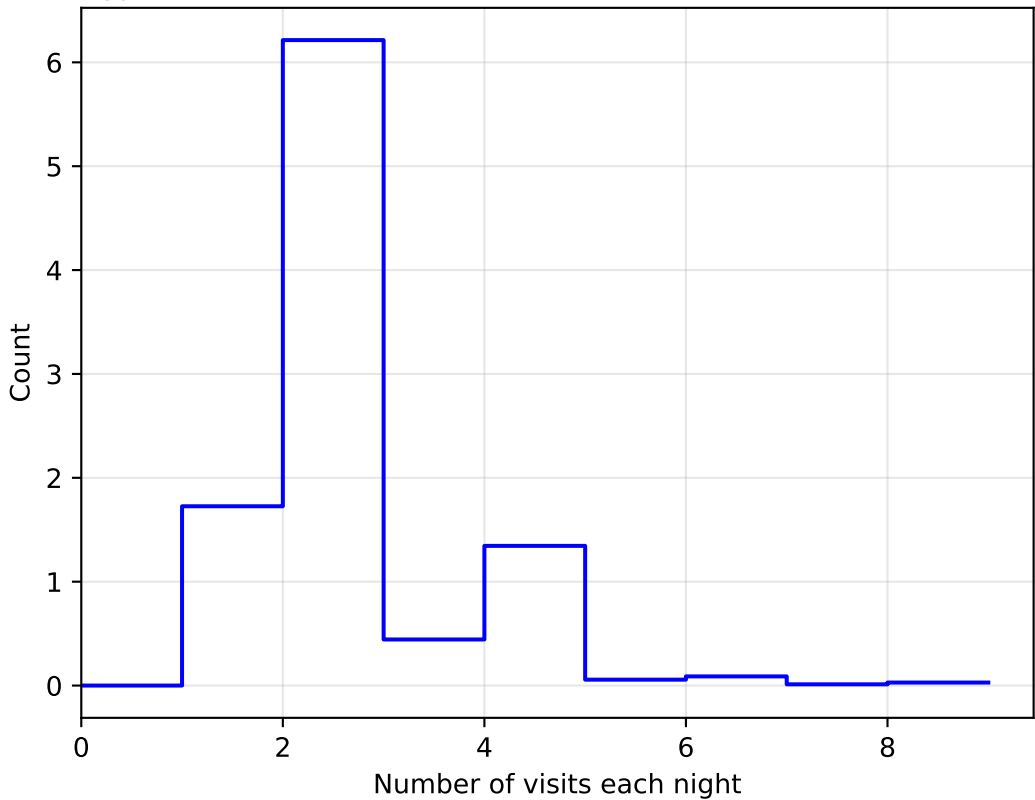
ddf_acor_sf25_lsf40_lsr10_v3.4_10yrs All sky: NVisitsPerNight 1e6
