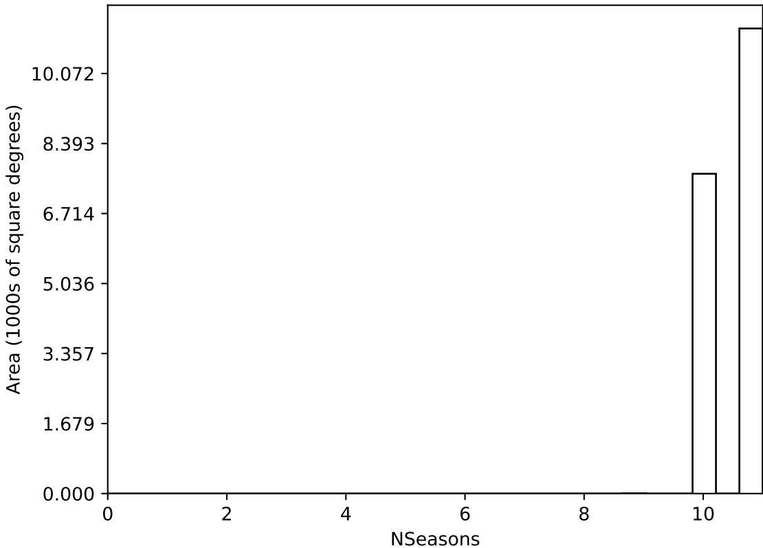
ddf_acor_sf25_lsf40_lsr10_v3.4_10yrs WFD all bands: NSeasons
