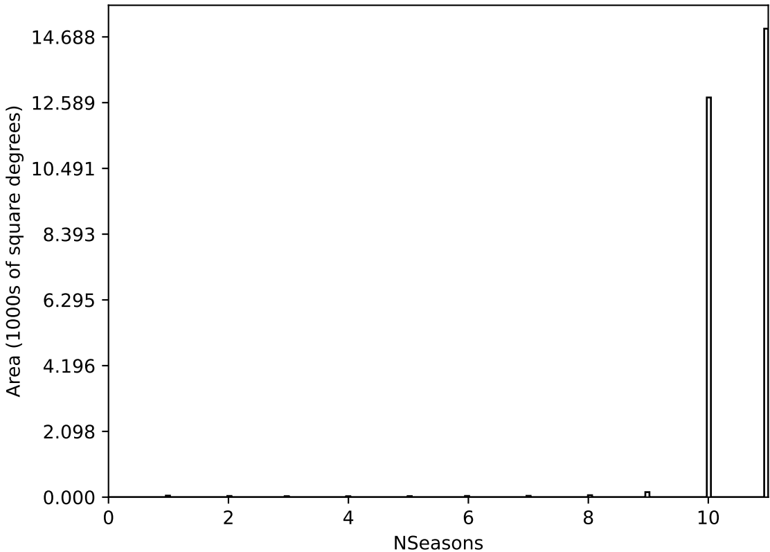
ddf_acor_sf25_lsf40_lsr10_v3.4_10yrs All sky all bands: NSeasons
