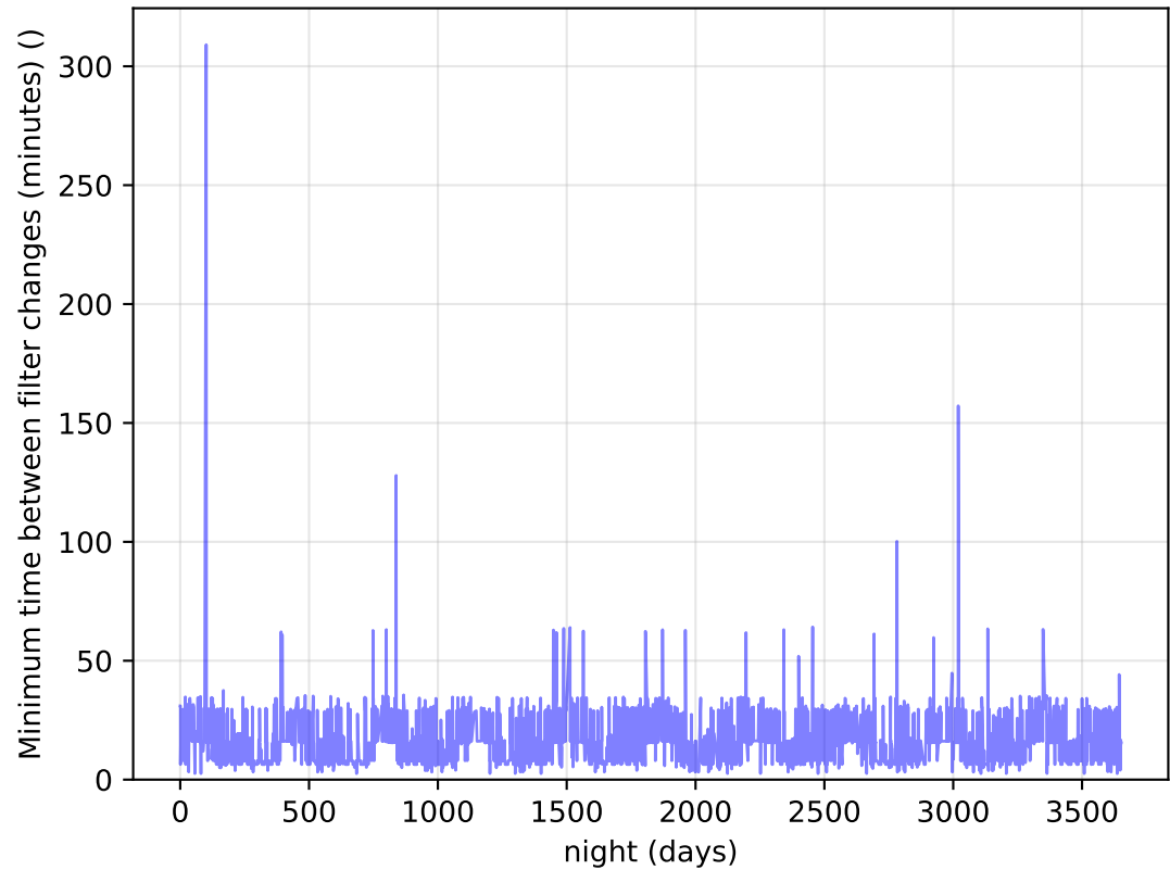
ddf_acor_sf25_Isf40_Isr10_v3.4_10yrs Per Night: Minimum time between filter changes (minutes)
