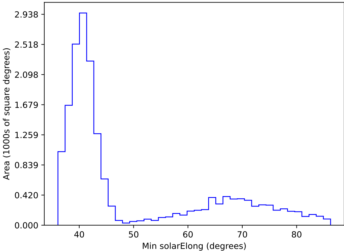
ddf_acor_sf25_lsf40_lsr10_v3.4_10yrs WFD z band: Min solarElong
