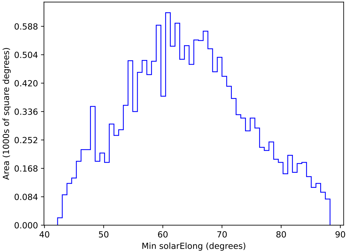
ddf_acor_sf25_lsf40_lsr10_v3.4_10yrs WFD y band: Min solarElong
