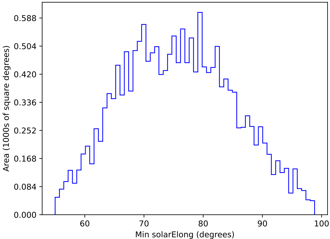
ddf_acor_sf25_lsf40_lsr10_v3.4_10yrs WFD u band: Min solarElong
