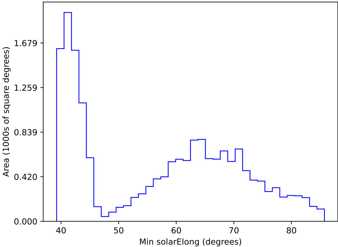
ddf_acor_sf25_lsf40_lsr10_v3.4_10yrs WFD r band: Min solarElong
